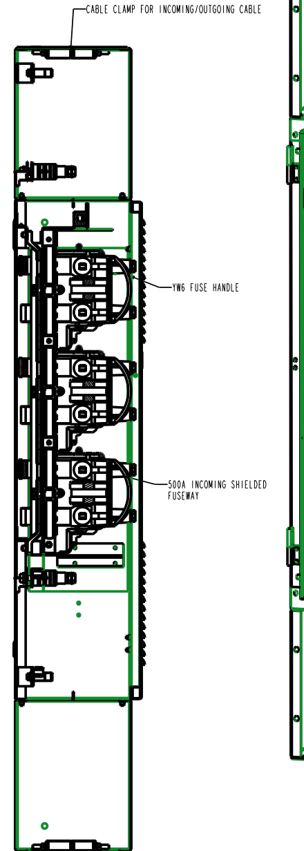
SECTION C-C SHOWING 500A INCOMING SHIELDED FUSEWAY
