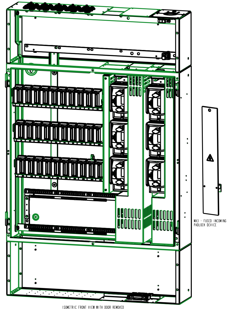
ISOMETRIC FRONT VIEW WITH DOOR REMOVED
