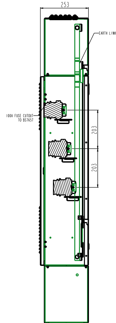
SECTION B-B SHOWING 100A FUSE CUTOUT
