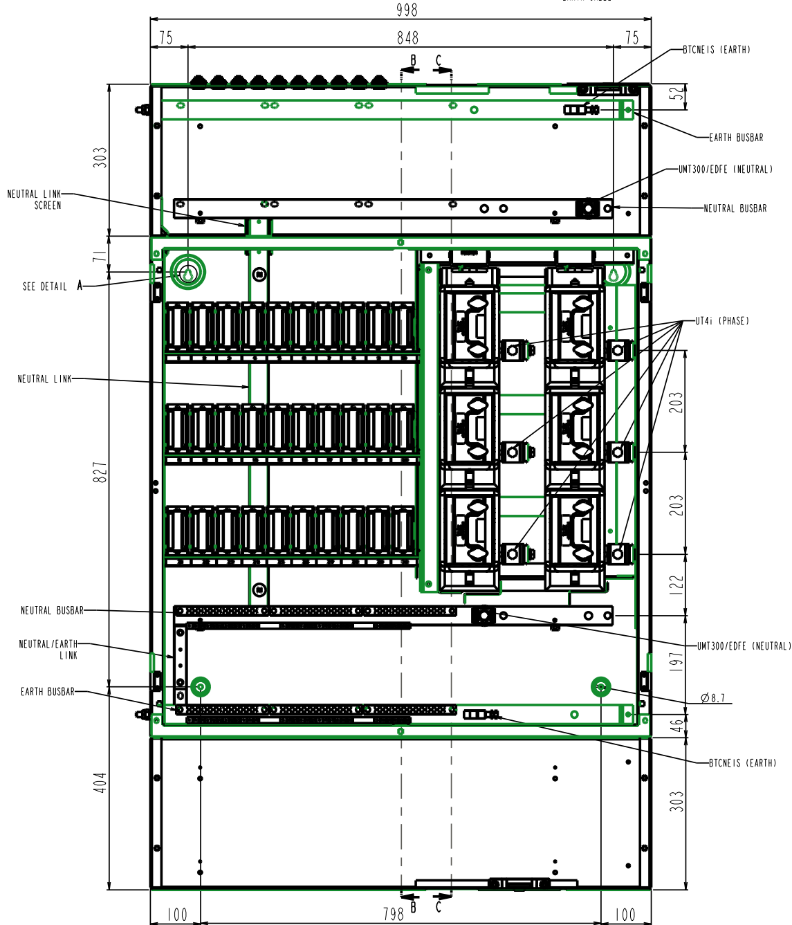
FRONT VIEW WITH DOOR AND INCOMING/OUTGOING CABLE SCREENS REMOVED
